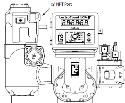
Figure 6: New Assembly
