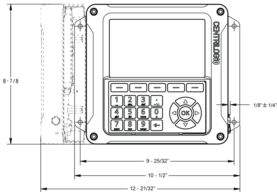
FRONT VIEW
